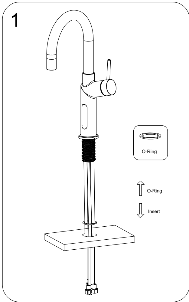
1. Insert the O-ring(B) over the hoses into tap shank, and mount the tap on the sink/Bencht top, see fig.1
