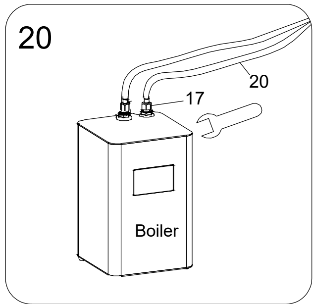
20. Connect 6mm dia hose(20) supplied from control box to quick fit connector(17) on the boiler filtered water in(blue), see fig.20
