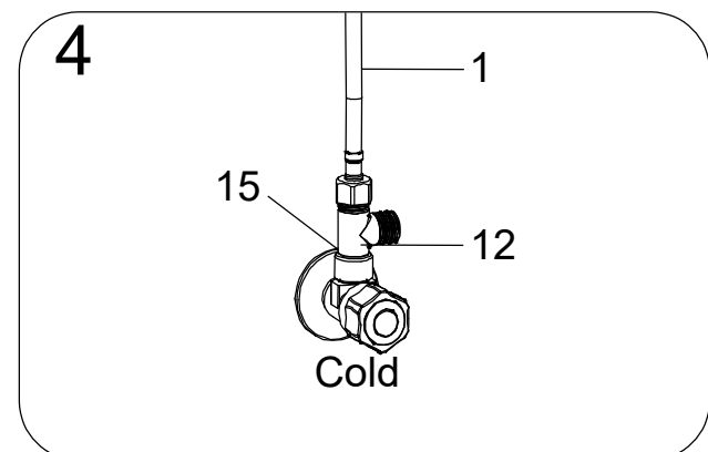
4. Add flow Restrictor(15) into T Adaptor where it connects to mains water. Side with small O-ring on flow restrictor faces towards mains water supply. Connect hose(1) onto T adaptor(12) tighten firmly, see fig.4
